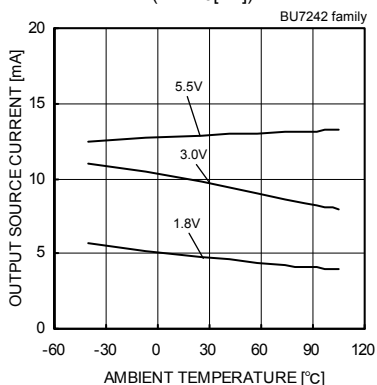
Fig. 79 Output Source Current - Ambient Temperature (VOUT=VDD-0.4[V])
