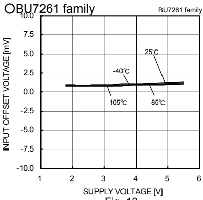
Fig. 13 Input Offset Voltage – Supply Voltage (V icm =V DD , V OUT =1.5[V])
