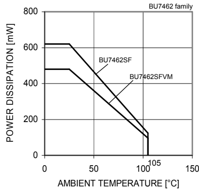
Fig. 117 Derating curve
