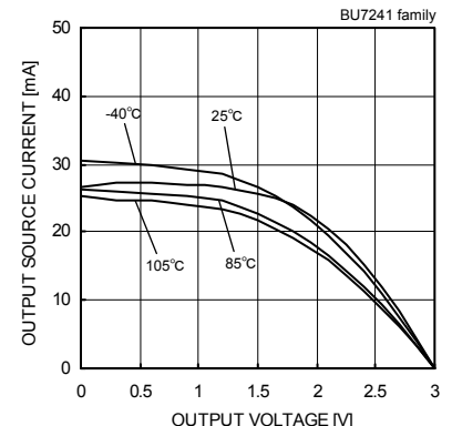
Fig. 55 Output Source Current - Output Voltage (VDD=3.0[V])
