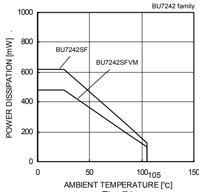
Fig. 71 Derating curve
