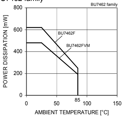
Fig. 116 Derating curve
